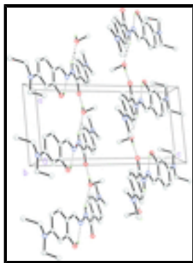
Fig. 2. Crystal packing of the title compound, viewed down the b axis. Intermolecular interactions are drawn as dashed lines.
